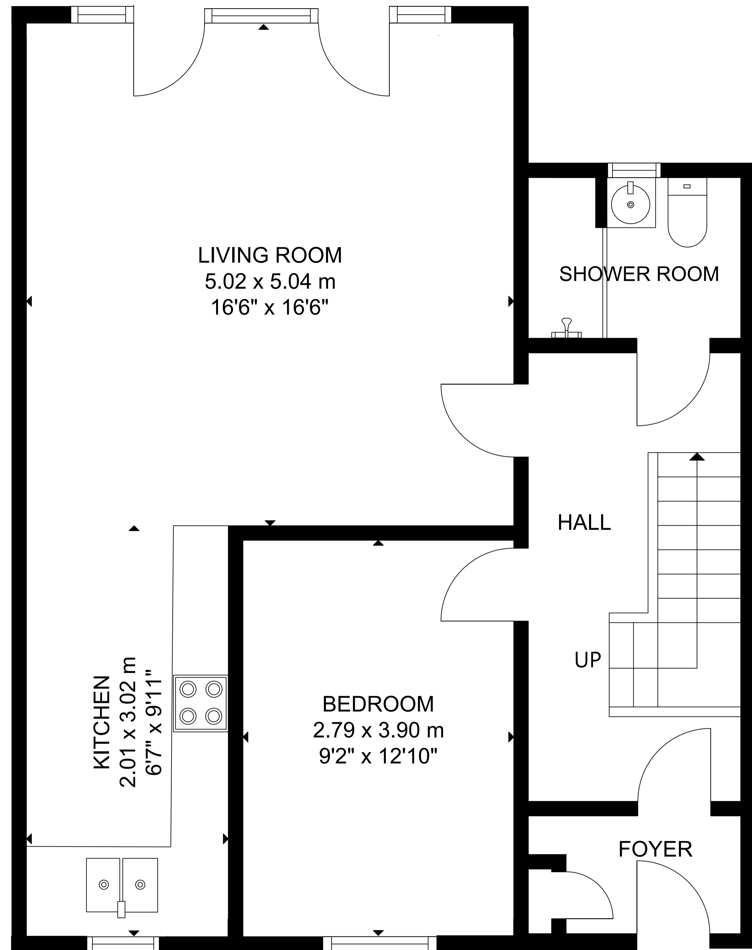
GROUND FLOOR
