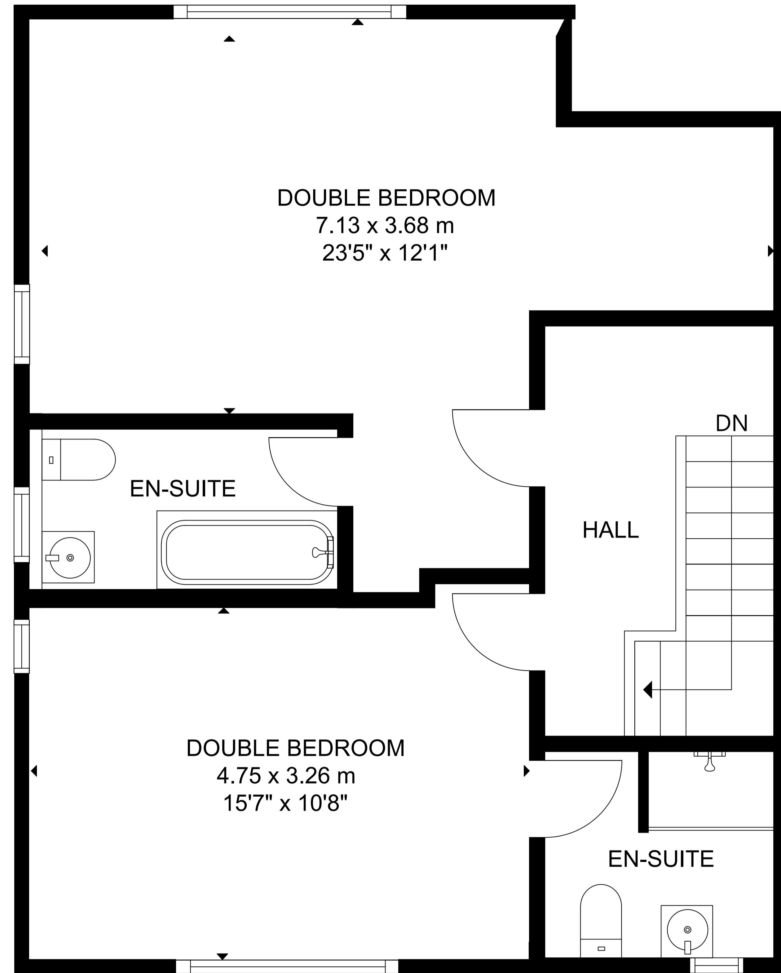
FIRST FLOOR
